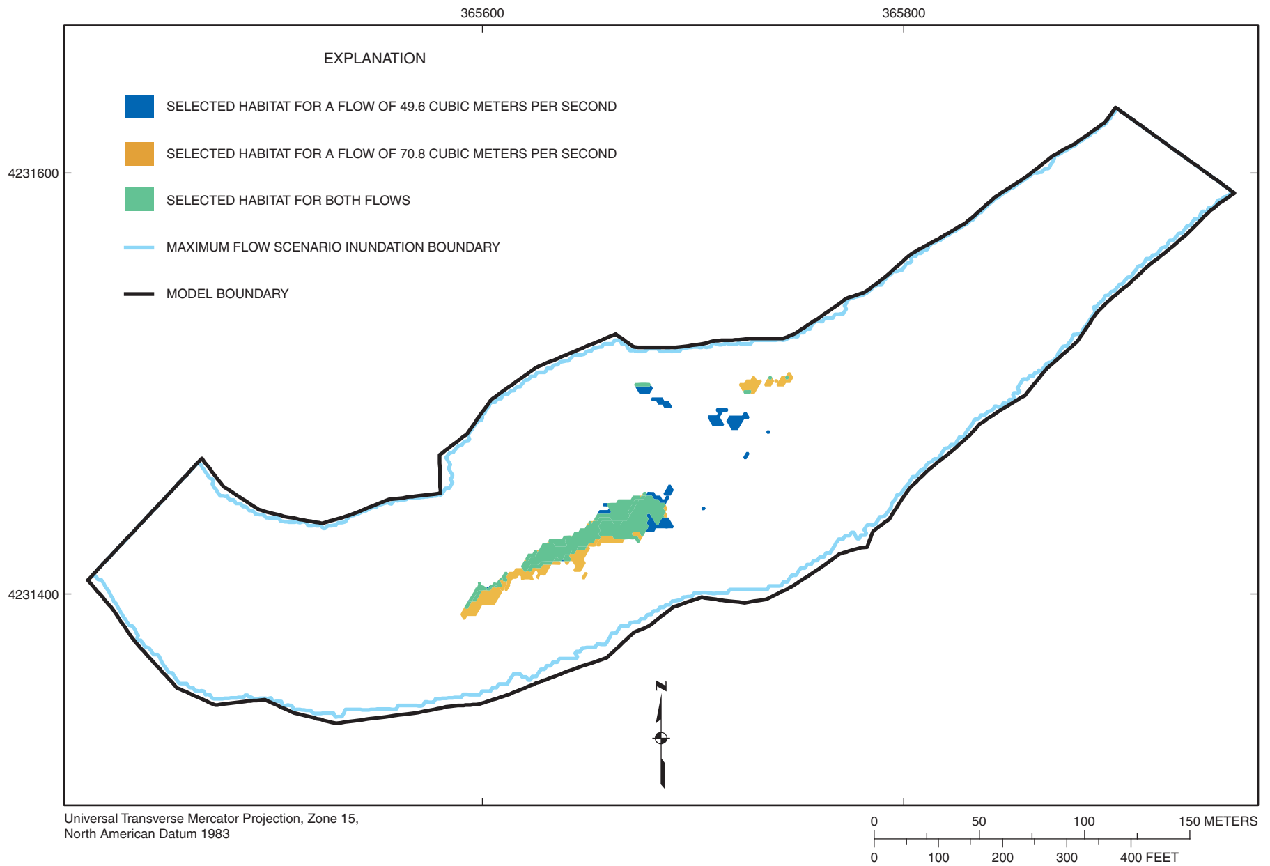
Figure 4-19. Selected habitat area distribution for habitat categories 4, 5 combined (slenderhead darter) at flows of 49.6 and 70.8 cubic meters per second at Marais des Cygnes River site MDC2.
